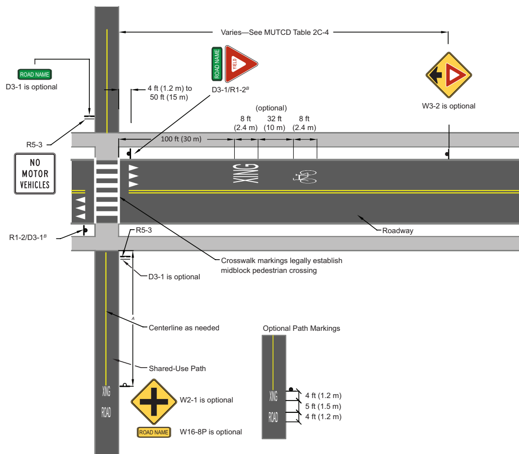
Notes: A Advance warning signs and solid centerline striping should be placed at the required stopping sight distance from the roadway edge, but not less than 50 ft (15 m). B D3-1 sign is optional, R1-2 sign is required. At multilane road crossings, the R1-5 series (Yield Here To/Stop Here for Pedestrians signs and markings, placed in advance of the crosswalk to reduce multiple-threat crashes) may be a more appropriate solution.
