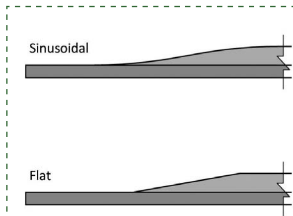
Figure 4-35. Examples of Bicycle-Friendly Approach Profiles for Speed Humps and Speed Tables
